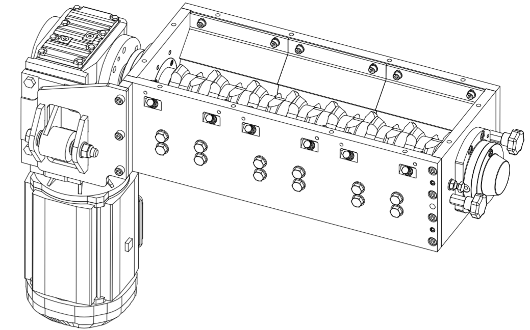
Shredder STS-B16.03_D
