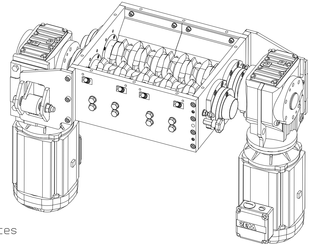
Shredder STS-B24.03_D
